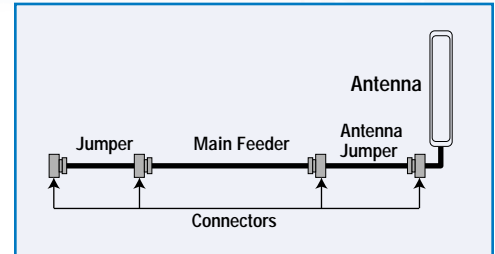
Figure 1. Typical transmission line system
